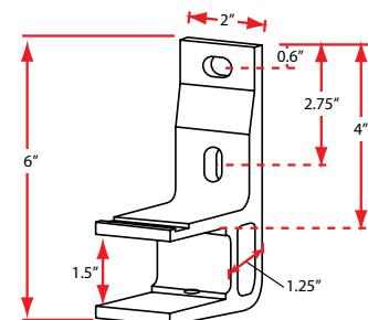
S / L series Wall Bracket
